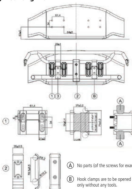
Front Fairing Mounting Kit
